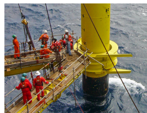
3. Suction operation and welding to bracing
